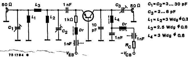
Test circuit for: G_{pb}
